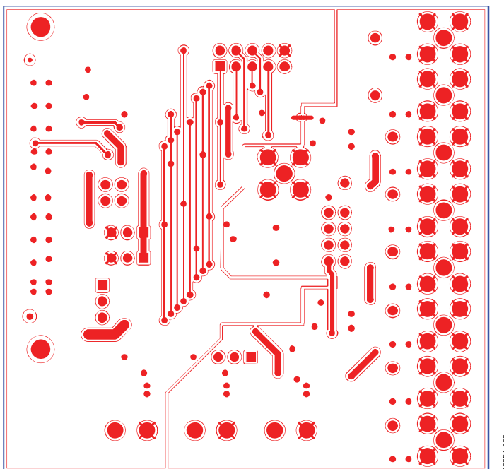
Figure 10. AD568x(R) Bottom Side Routing
